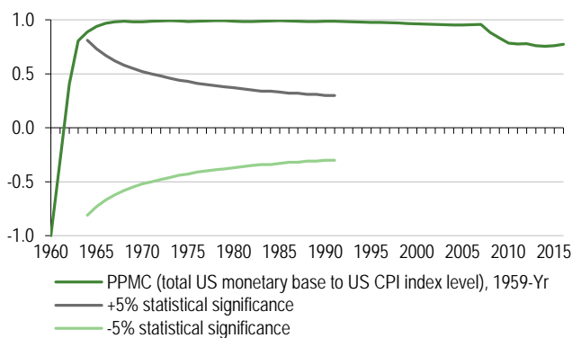
Exhibit 164: Correlation (PPMC), total monetary base to US CPI level, 1959-2016
