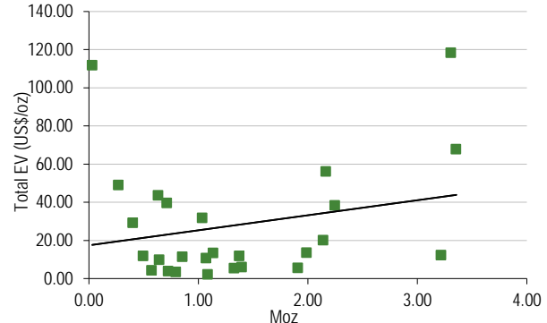
Exhibit 21: Graph of resource size (Moz) vs resource multiple (US$/oz) for ASX-listed gold explorers
