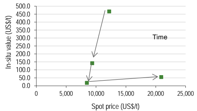
Exhibit 93: In-situ value of vanadium resources vs spot price of vanadium, 2014-17
