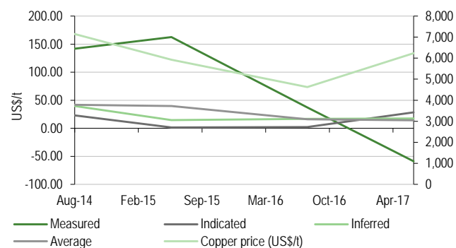
Exhibit 68: In-situ value of copper resources vs spot price of copper, by category, 2014-17
