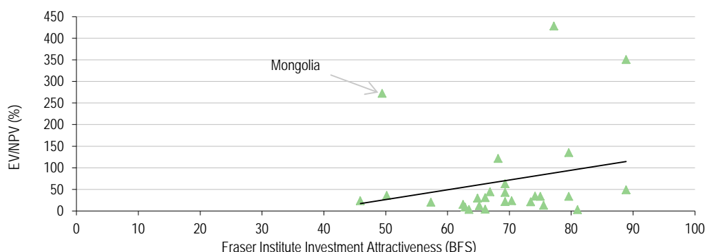
Exhibit 147: Company EV as percent of attributable project NPV (%) vs Fraser Institute Mining Investment Attractiveness Index score for projects at BFS level only
