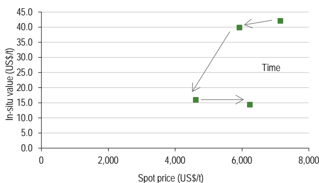
Exhibit 69: In-situ value of explorers' copper resources vs spot price of copper, 2014-17
