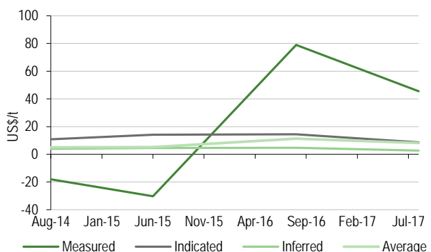
Exhibit 58: In-situ value of nickel laterite resources vs spot price of nickel, by category, 2014-17
