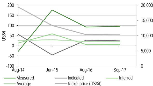
Exhibit 57: In-situ value of nickel sulphide resources vs spot price of nickel, by category, 2014-17
