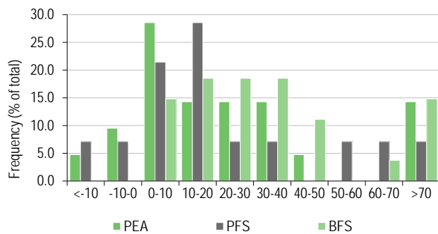
Exhibit 131: Company EV as percent of attributable project NPV (%), by study type, density histogram
